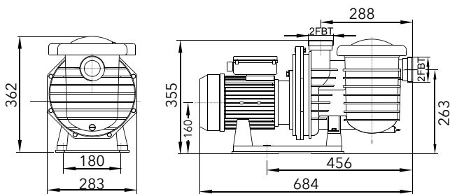
SMP - 20/30
